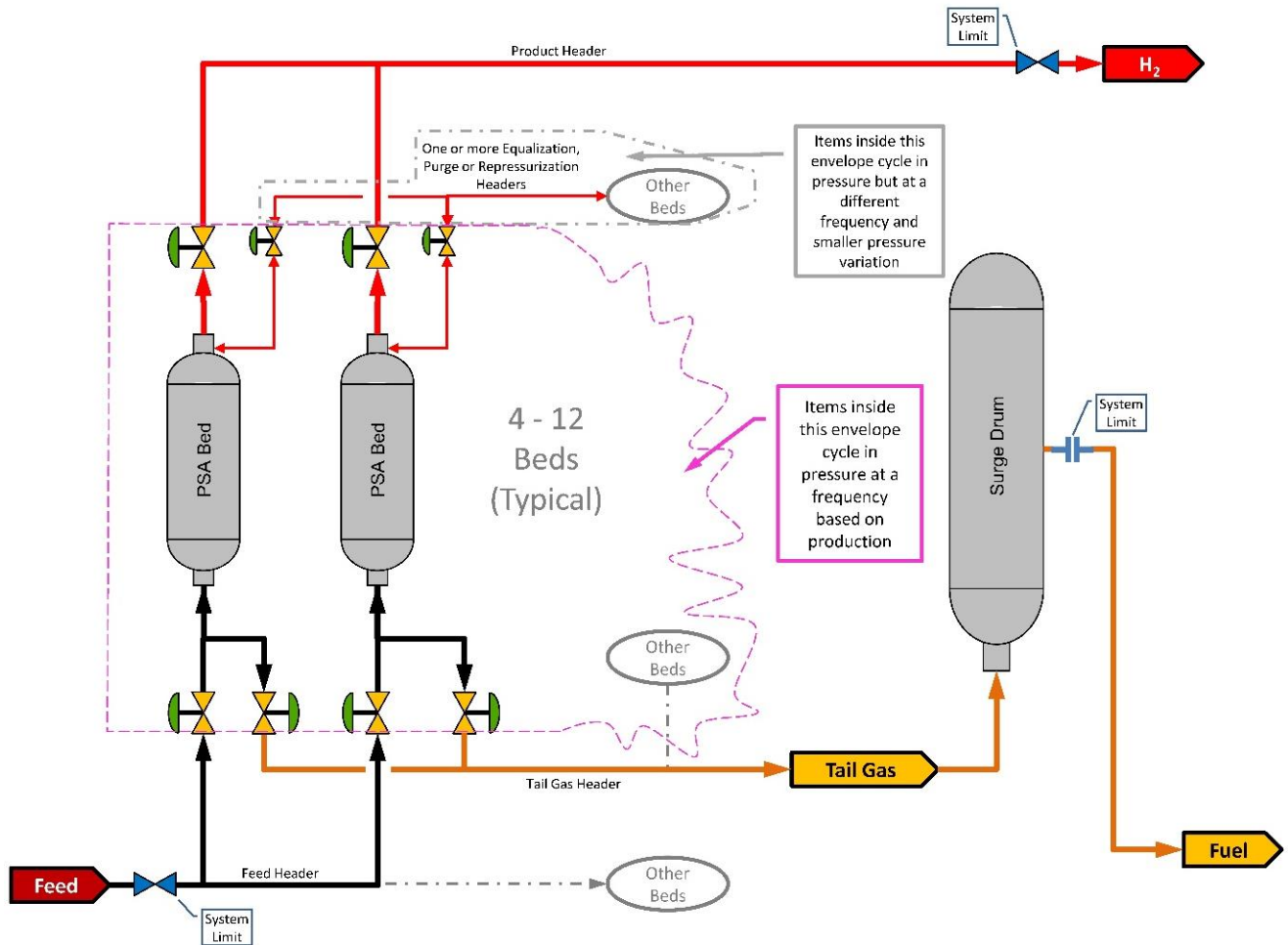
Figure 1—PSA system schematic
